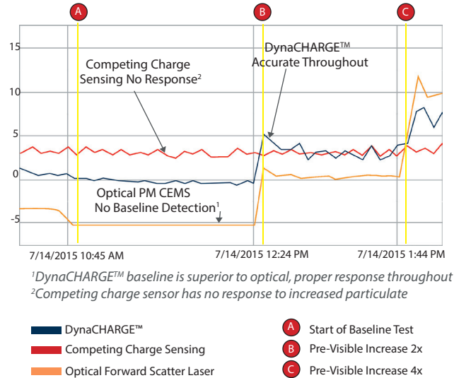
Figure 1 – Plant A: Low-Level Response Testing
